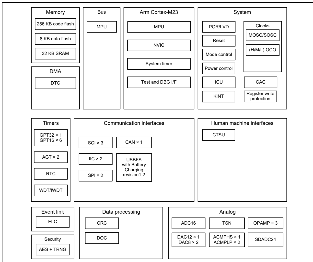
Figure 1.1 Block diagram
