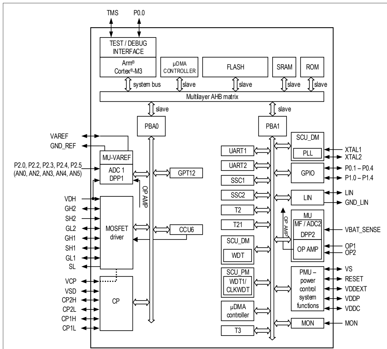
Figure 1 Block diagram
