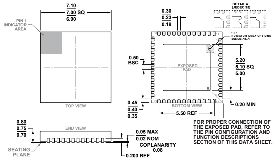
Figure 45. 48-Lead Lead Frame Chip Scale Package (LFCSP)
