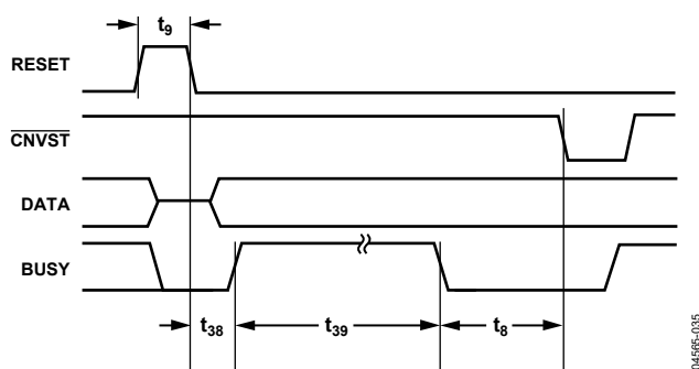
Figure 33. RESET Timing
