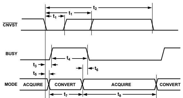
Figure 32. Basic Conversion Timing
