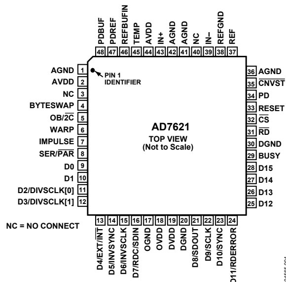
Figure 5. 48-Lead LQFP Pin Configuration
