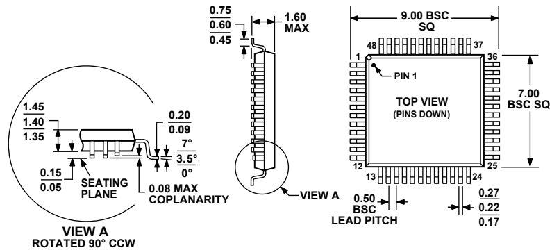
Figure 44. 48-Lead Low Profile Quad Flatpack (LQFP)
