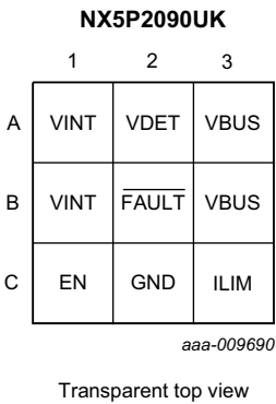
Fig 4. Ball mapping for WLCSP9
