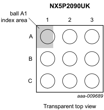
Fig 3. Pin configuration WLCSP9 package
