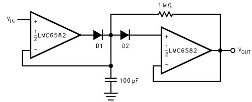
FIGURE 18. Low Voltage Peak Detector
