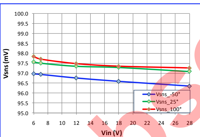
SENSE VOLTAGE VS. V_{IN}
