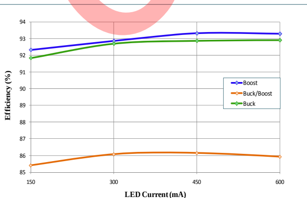
SYSTEM EFFICIENCY vs. LED CURRENT
