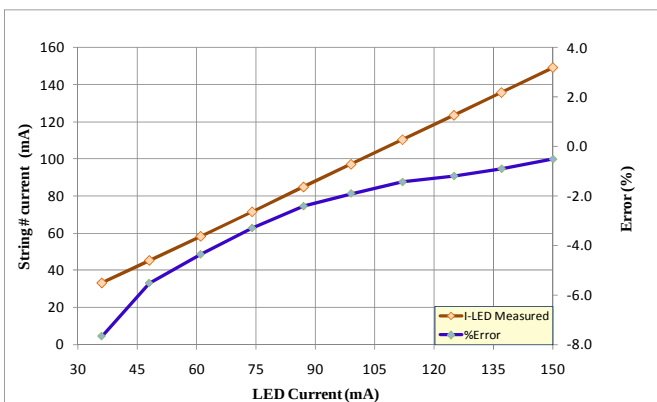
STRINGS CURRENT ACCURACY vs. LED CURRENT (ADIM BOOST MODE)
