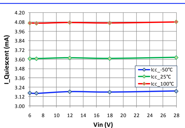
QUIESCENT CURRENT VS. V_{IN}
