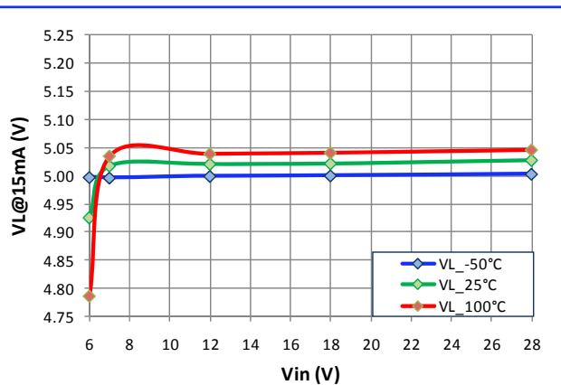
VL@15mA LOAD VS. V_{IN}
