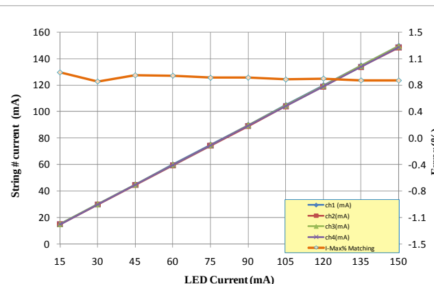
STRING CURRENT MATCHING vs. LED CURRENT (BUCK)
