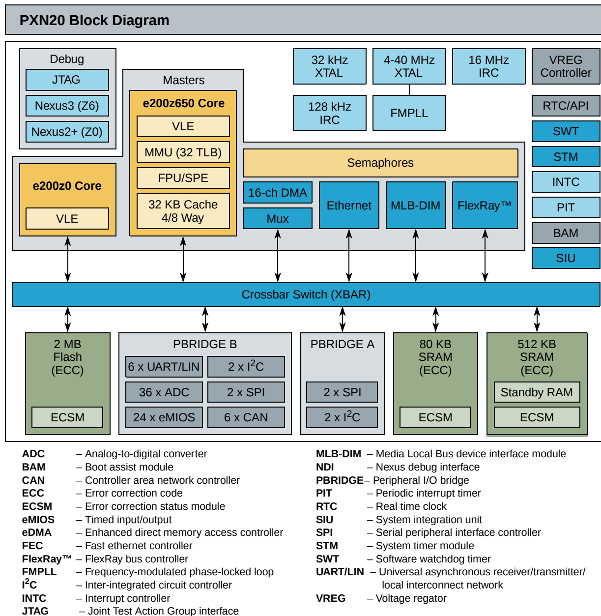
Figure 2. PXN20 block diagram
