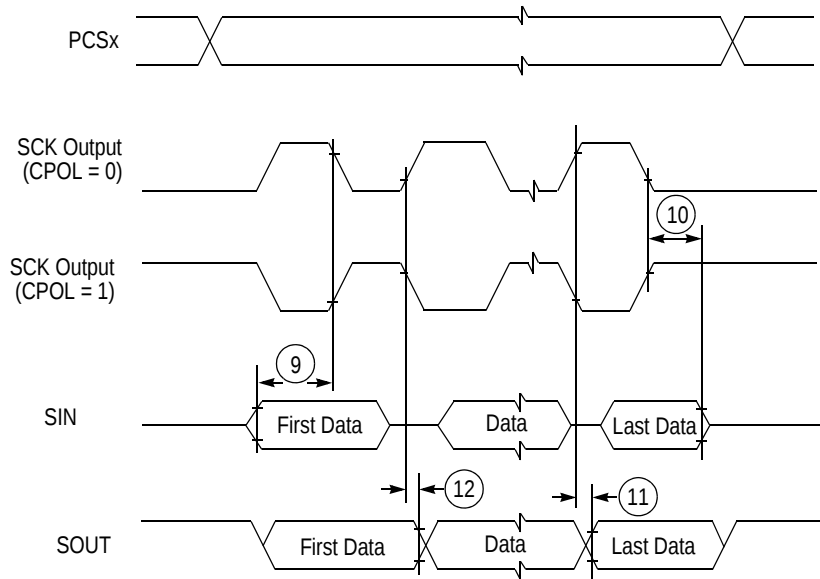
Figure 15. DSPI classic SPI timing — Master, CPHA = 1
