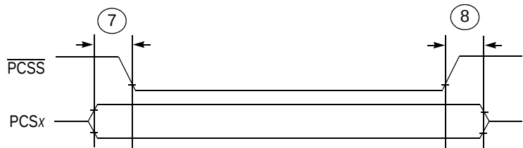
Figure 22. DSPI PCS strobe ( \overline{\text{PCSS}} ) timing
