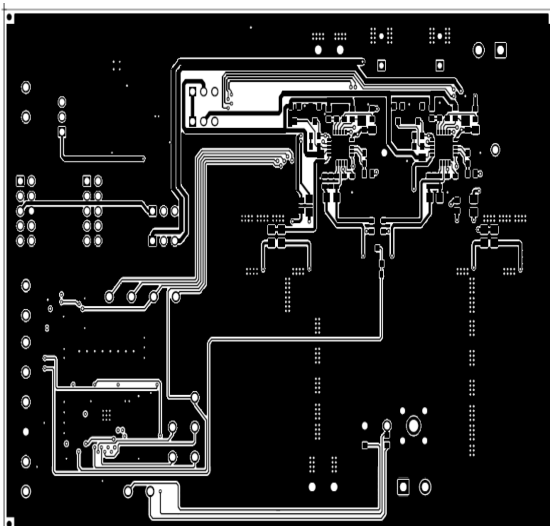
Figure 17. UCD9112EVM PCB Bottom Layer (Solder Side)
