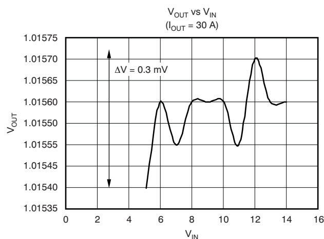
Figure 4. Line Regulation
