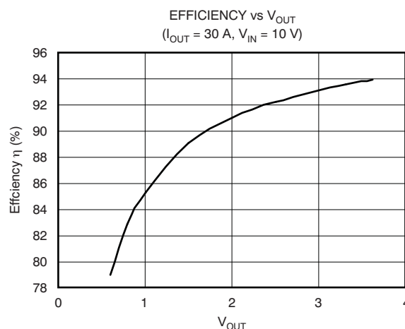
Figure 7. Efficiency \eta vs V_{OUT}
