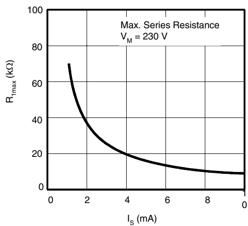
Figure 10. Maximum Resistance of R_1
