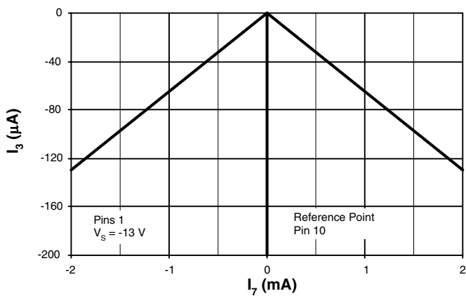
Figure 9. Mains Voltage Compensation
