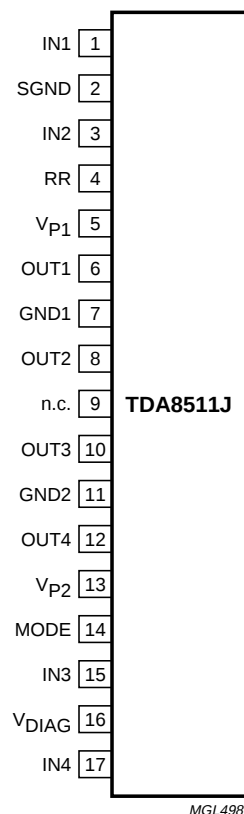
Fig.2 Pin configuration.
