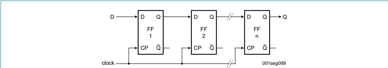
Fig 7. N-stage shift register
