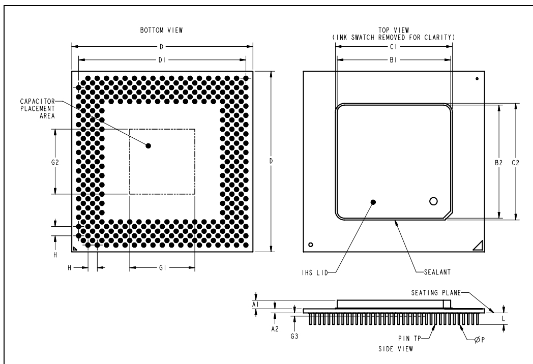
Figure 22. Package Dimensions
