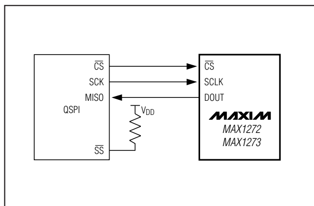
Figure 11. QSPI Connections
