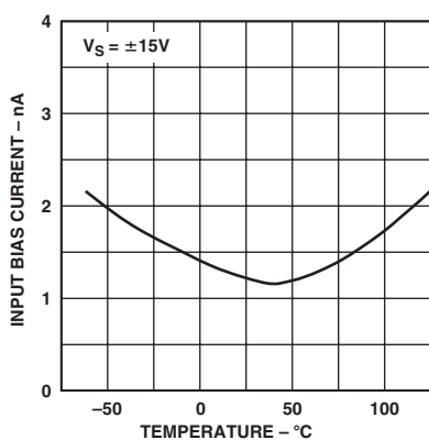
TPC 11. Input Bias Current vs. Temperature
