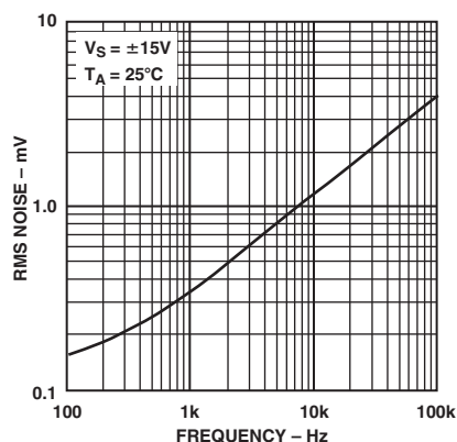
TPC 13. Input Wideband Noise vs. Bandwidth (0.1 Hz to Frequency Indicated)
