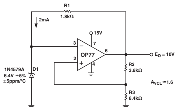
Figure 13. High Stability Voltage Reference
