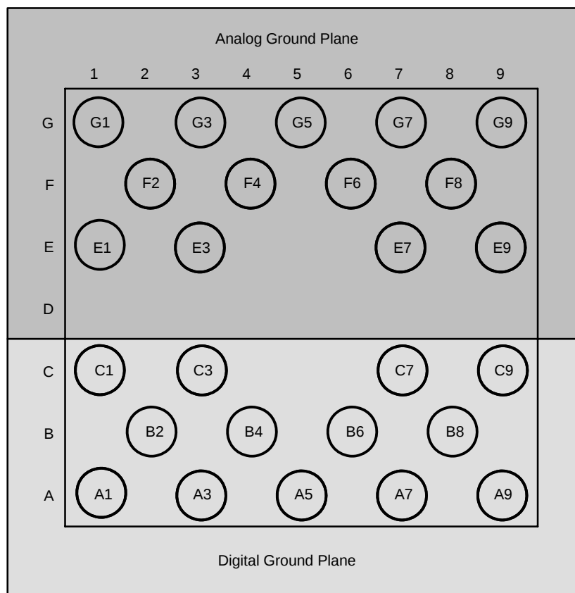
Figure 3. Proposed Ground Plane Positioning (soldering footprint view)
