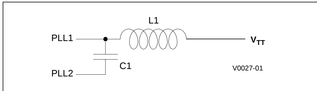
Figure 6. PLL Filter
