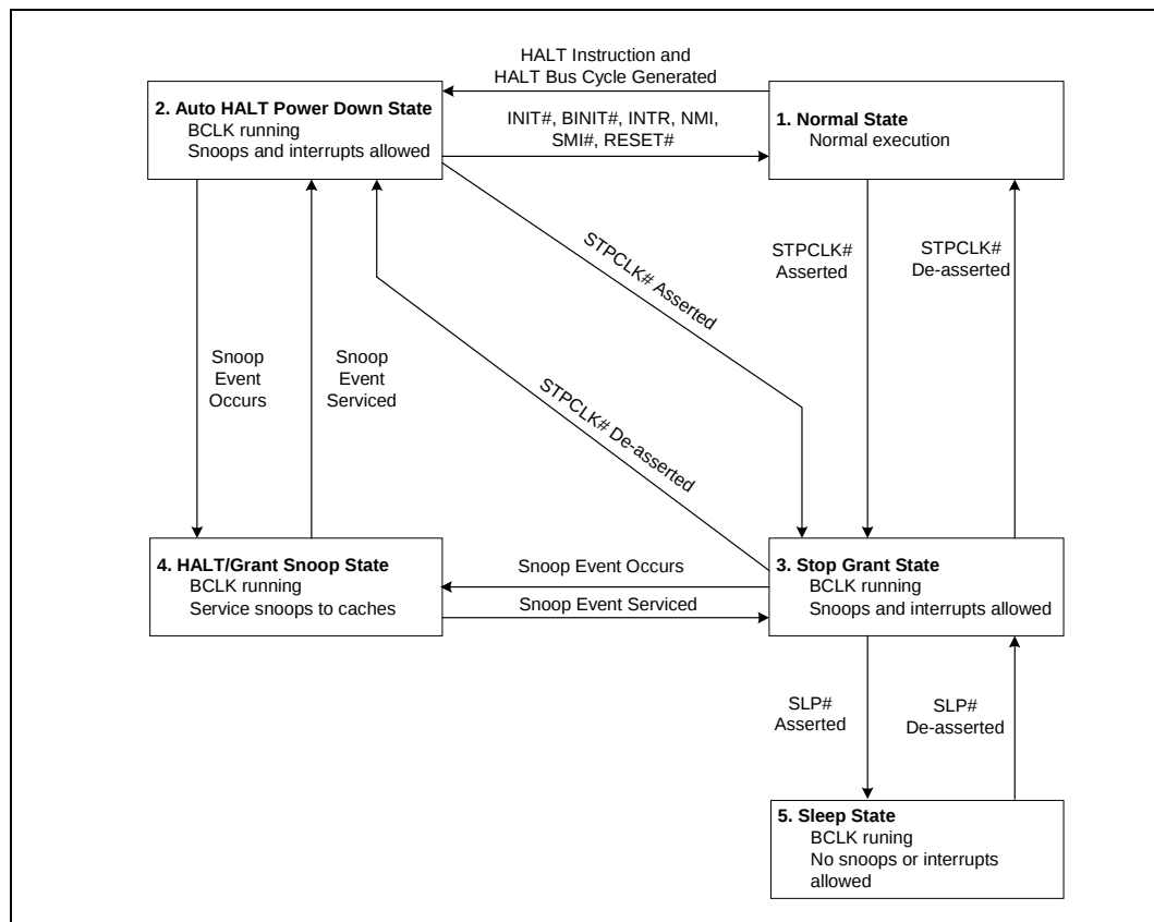
Figure 2. Stop Clock State Machine
