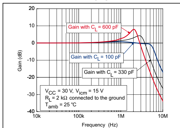
Figure 18. Frequency response for different capacitive loads at V_{CC} = 30 V, V_{icm} = 15 V and T = 25 °C
