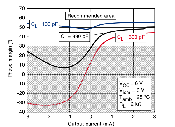
Figure 19. Phase margin vs. output current, at V_{CC} = 6 V, V_{icm} = 3 V and T = 25 °C
