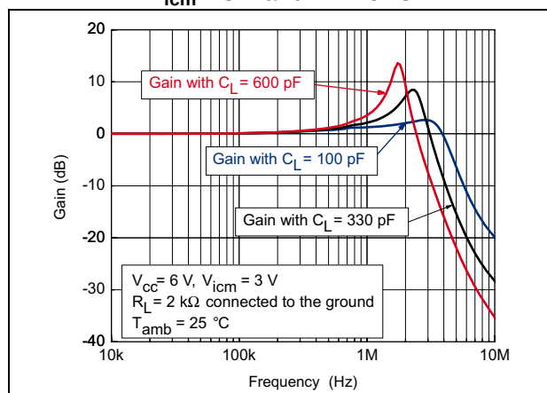
Figure 16. Frequency response for different capacitive loads at V_{CC} = 6 V, V_{icm} = 3 V and T = 25 °C
