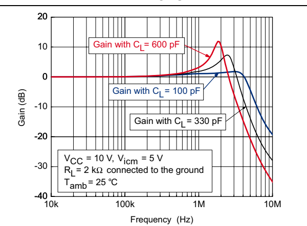
Figure 17. Frequency response for different capacitive loads at V_{CC} = 10 V, V_{icm} = 5 V and T = 25 °C
