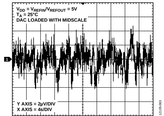
Figure 26. 0.1 Hz to 10 Hz Output Noise Plot, External Reference
