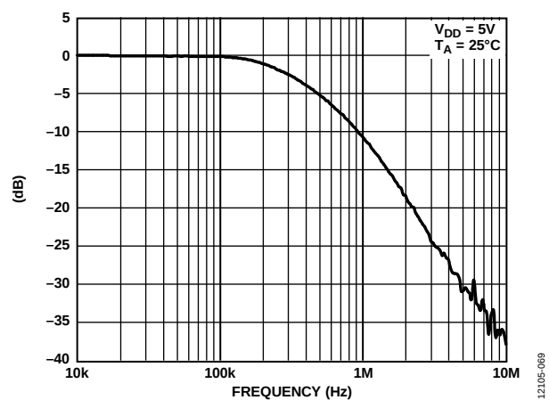
Figure 31. Multiplying Bandwidth
