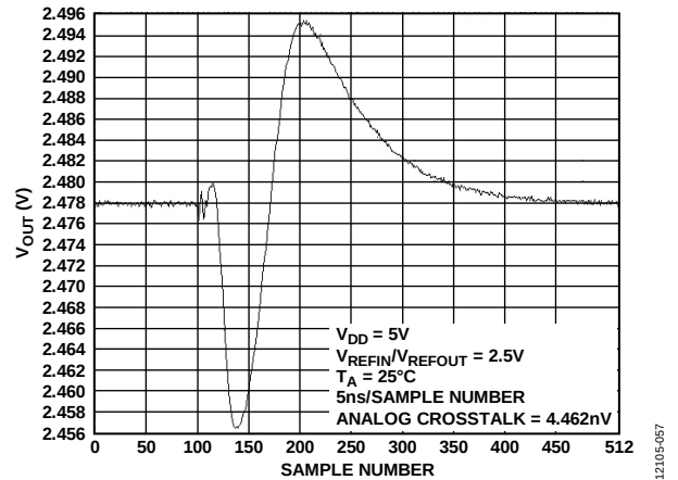
Figure 25. Analog Crosstalk, Internal Reference
