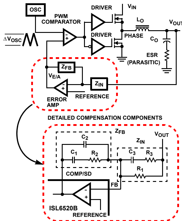
FIGURE 4. VOLTAGE-MODE BUCK CONVERTER COMPENSATION DESIGN
