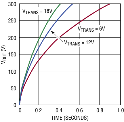
3A Charging Time
