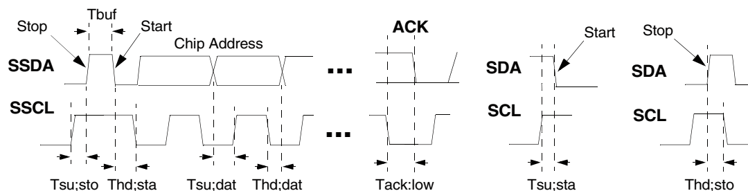
Figure 11. SSDA/SSCL Timing
