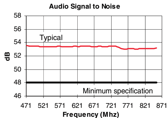
Figure 5. Typical performance—Audio
