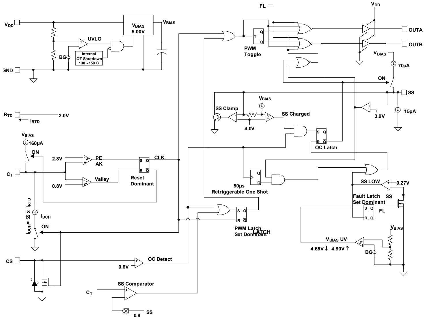
Figure 1. Block Diagram
