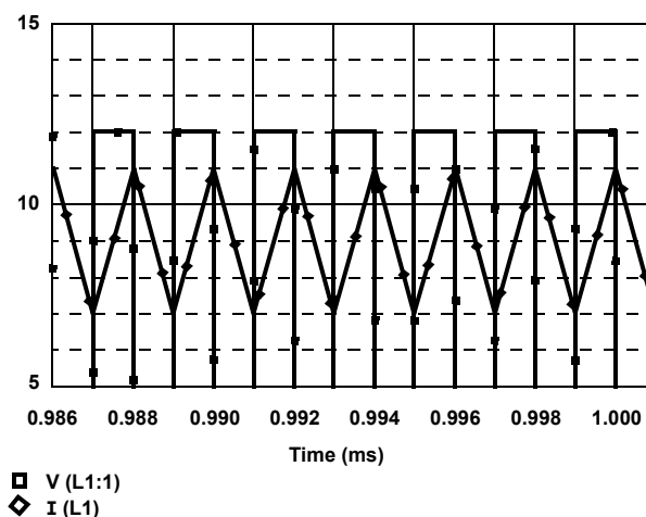
Figure 17. Secondary Winding Voltage and Inductor Current During Current Limit Operation
