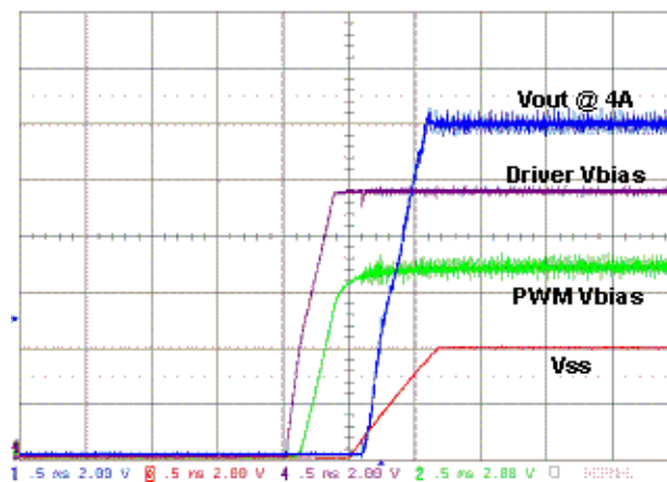
Figure 25. Output Soft-Start
