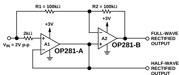
Figure 41. Single Supply Full- and Half-Wave Rectifiers Using an OP281
