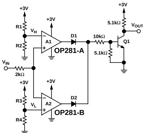
Figure 39. Using the OP281 as a Window Comparator
