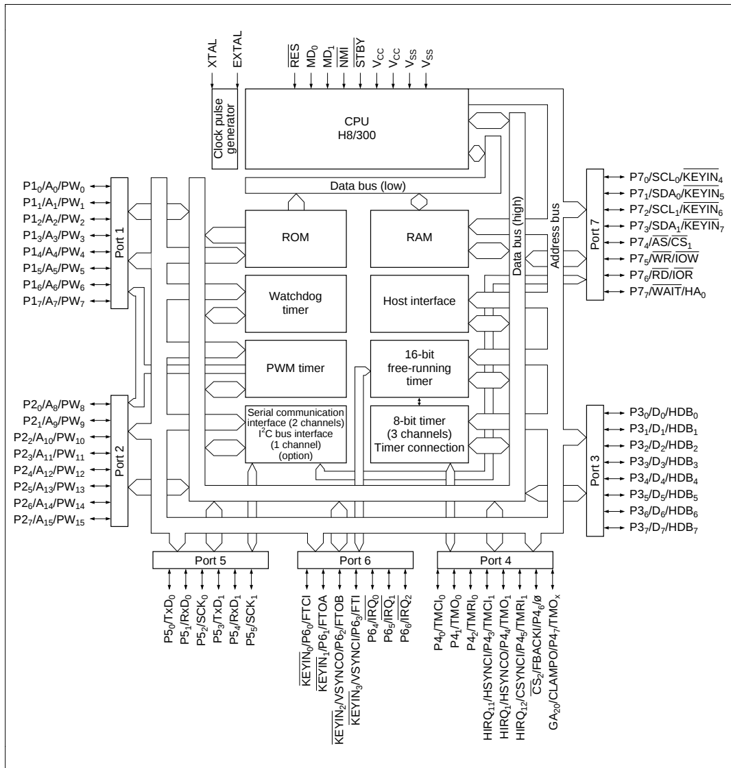
Figure 1-1 Block Diagram
