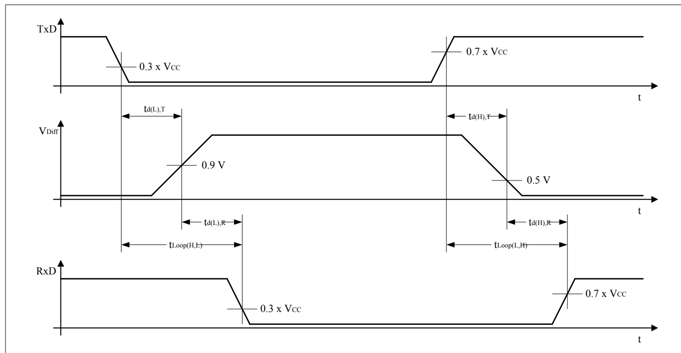
Figure 14 Timing diagram for dynamic characteristics
