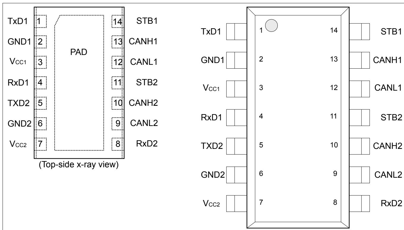
Figure 2 Pin configuration
