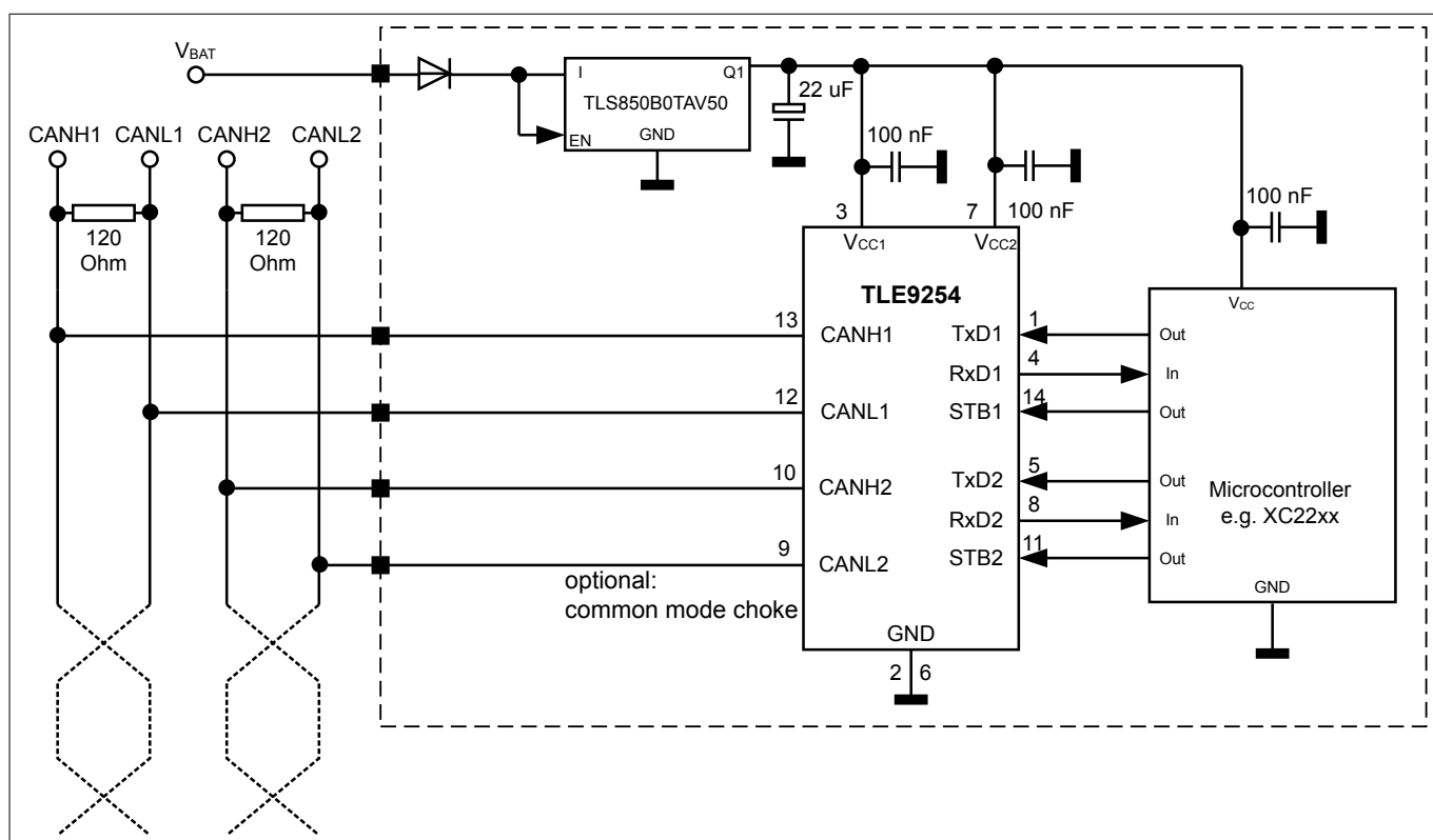
Figure 16 Application circuit
