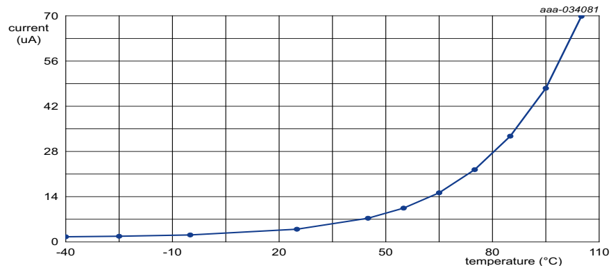
Fig 10. Power-down mode: Typical supply current I_{DD} versus temperature for different supply voltages VBAT_DCDC
