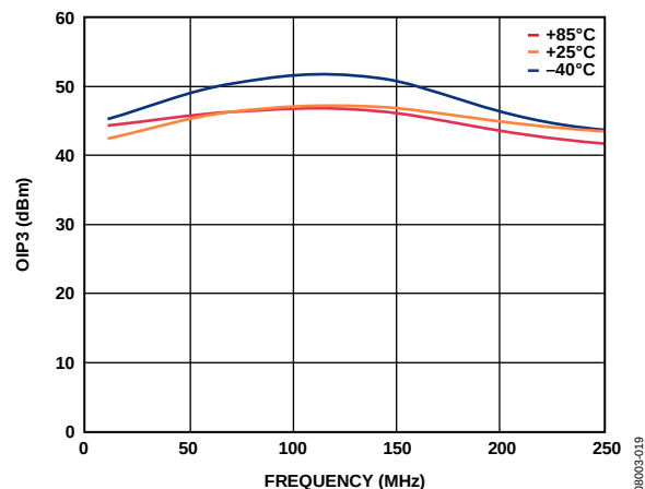
Figure 10. Output Third-Order Intercept vs. Frequency, Over Temperature, Output Level at 2 V p-p Composite, R_L = 200\ \Omega
