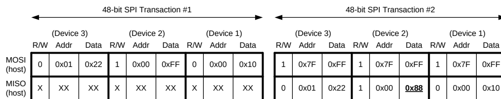
Figure 12. SPI Daisy-Chain Read and Write Example
