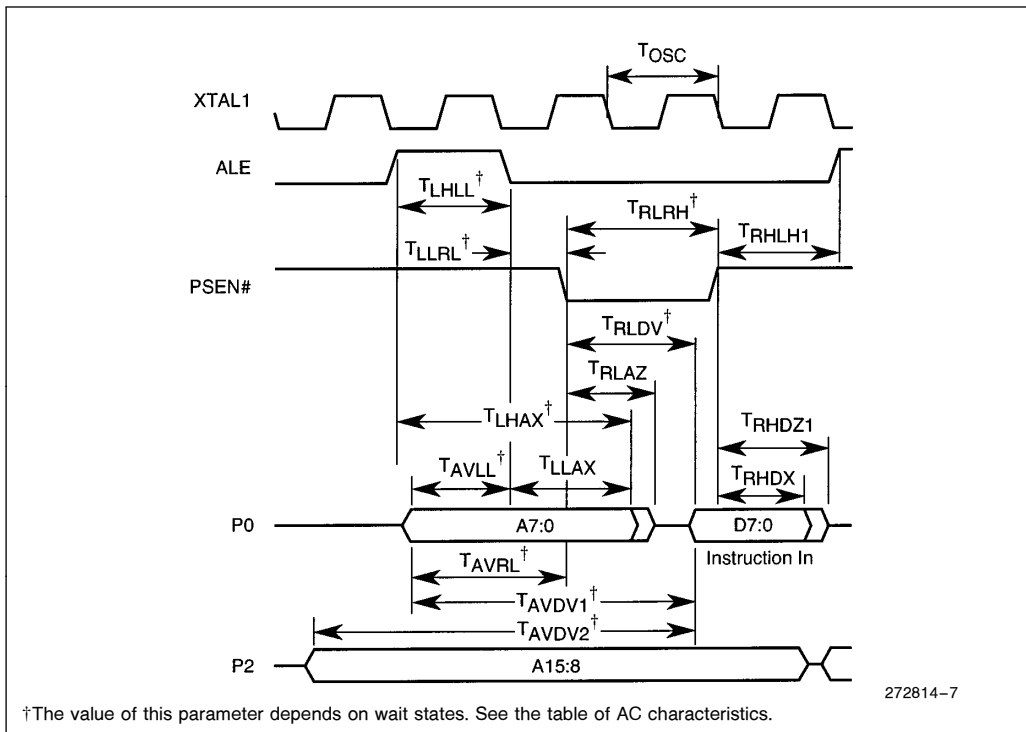
Figure 9. External Instruction Bus Cycle in Nonpage Mode
