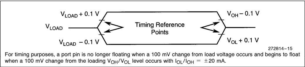
Figure 17. Float Waveforms
