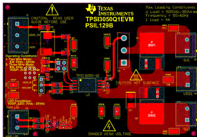
Figure 9-13. Top Layer
