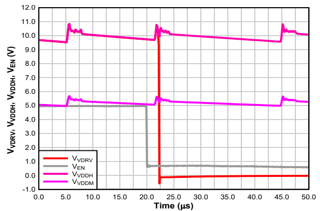
Figure 6-5. t LH_VDRV , Three-Wire Mode
