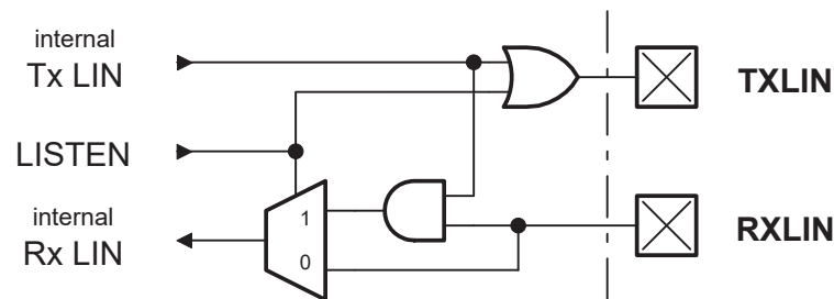
Figure 22-6. Listening mode.
