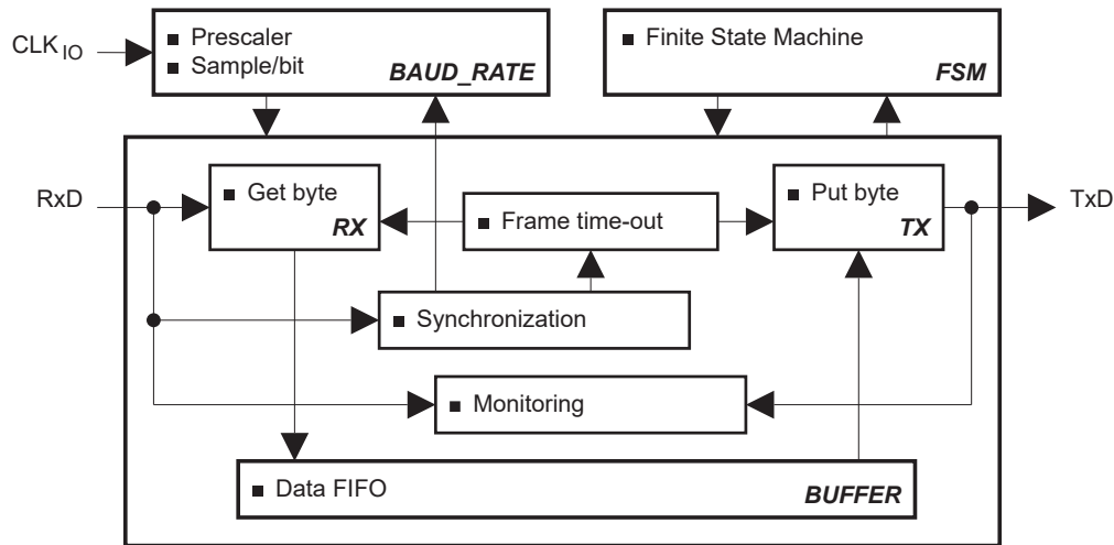
Figure 22-4. LIN/UART controller block diagram.
