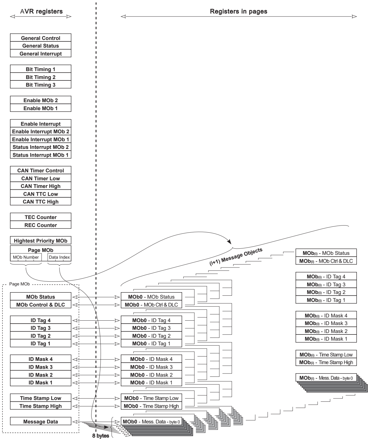
Figure 21-15. Registers organization
