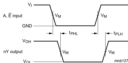
Fig. 3. The input A, \bar{E} to output nY propagation delays
