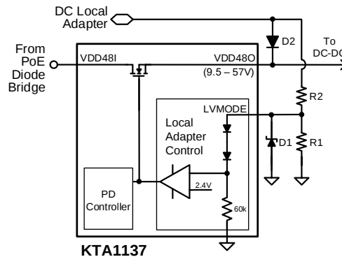
Figure 19. LVMODE Implementation
