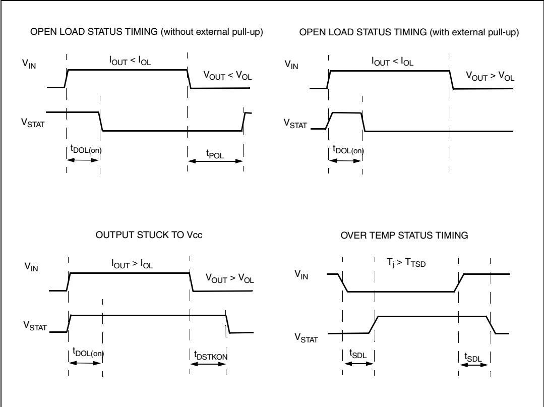
Figure 4. Status timings
