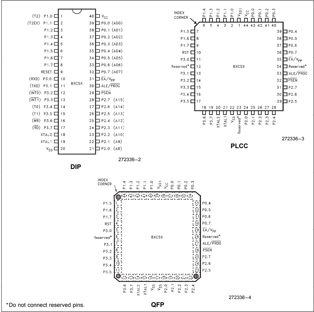
Figure 2. Pin Connections
