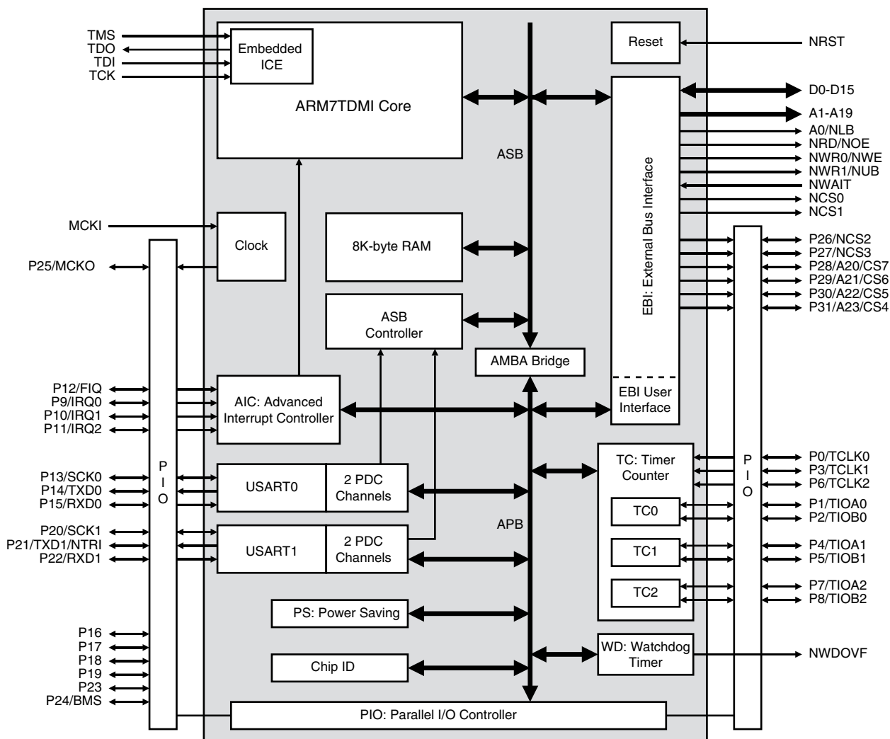
Figure 4-1. AT91M40800
