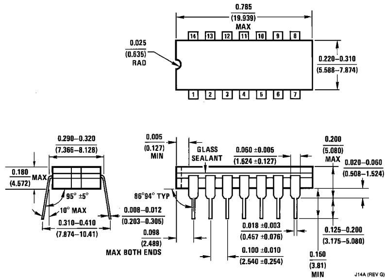
14-Lead Ceramic Dual-In-Line Package (J) Order Number 54LS74DMQB or DM54LS74AJ Package Number J14A
